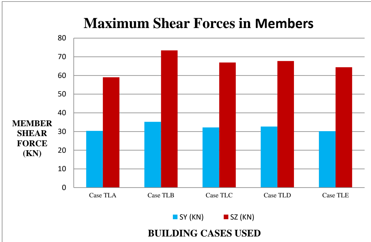
Fig.13: Comparative representation of Maximum Shear Forces in Members obtained in all Cases for Tower
