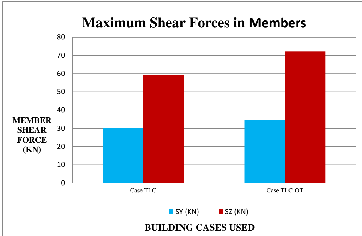
Fig. 27: Comparative representation of Maximum Shear Forces in Members obtained in Worst Case and Erected Case for Tower
